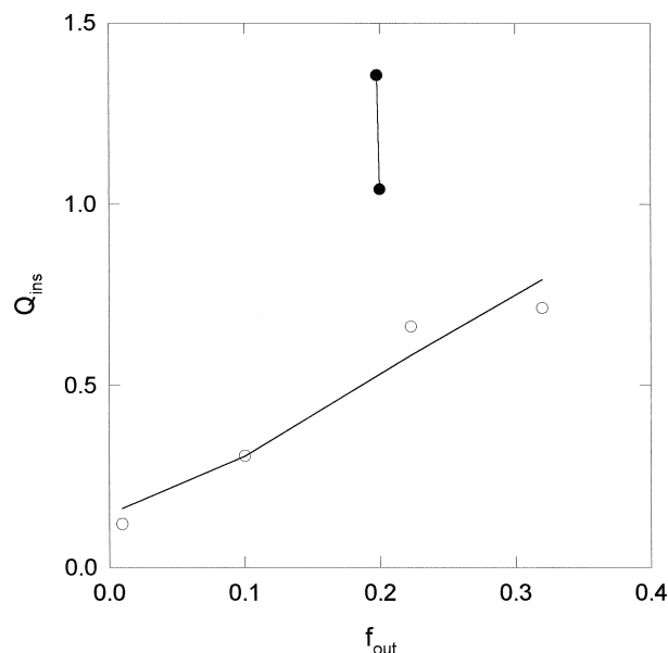
Fig. 7. The results of the all-or-none experiment using squalamine and PC LUVs. The results at low PC concentrations indicate a graded leakage mechanism. Above approximately 10 \mu M lipid, the experimental data deviates from expected, in parallel to the leakage results shown in Fig. 5. Open circles: 0.6–6 \mu M PC; Closed circles: 15–40 \mu M PC.
