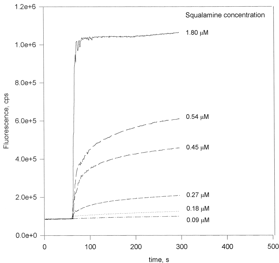
Fig. 2. The kinetics of carboxyfluorescein leakage from PG LUVs. Squalamine was added to PG LUVs (phospholipid concentration = 4.9 \mu M) to the final concentration indicated on the Figure, and the increase in CF fluorescence recorded. The fluorescence units are recorded in counts per second.
